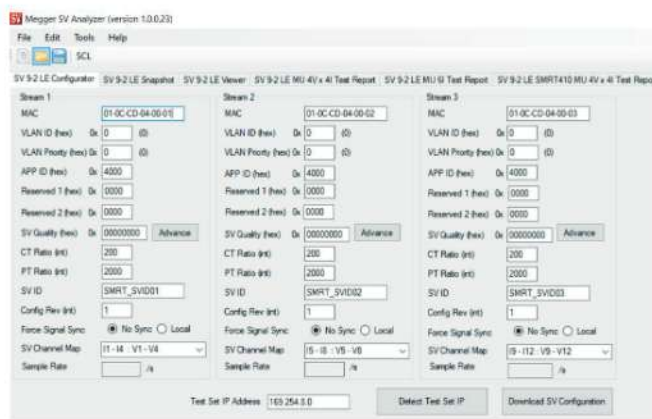
Megger Sampled Values Configurator
