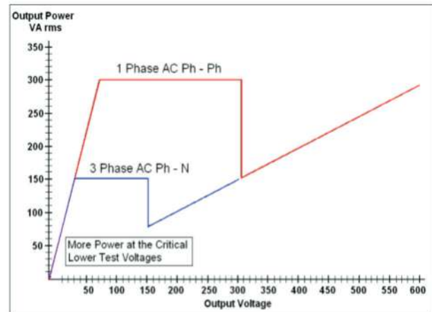
"PowerV" Voltage Amplifier Output Power Curve
